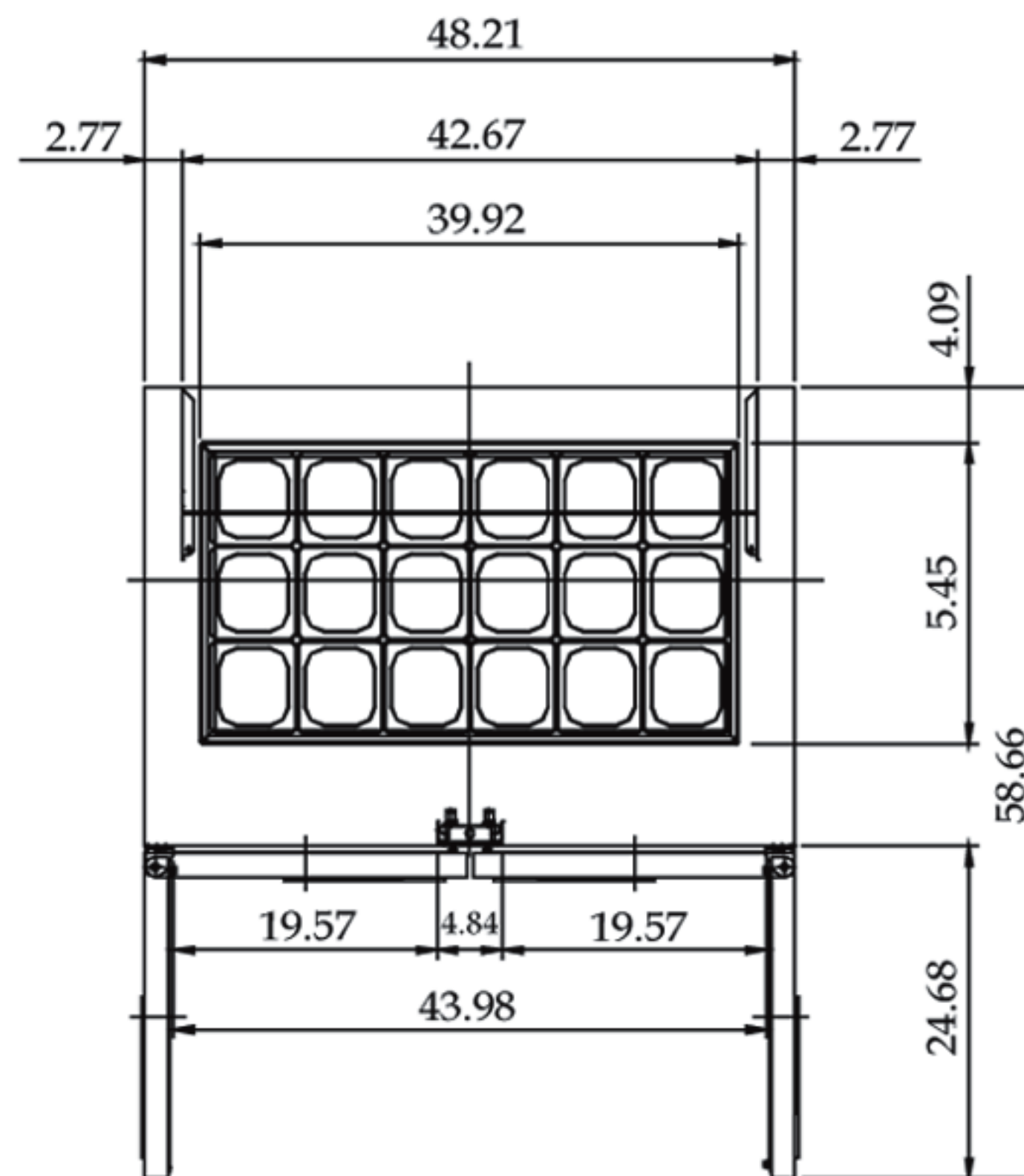
TST-48SD-18 PLAN VIEW
