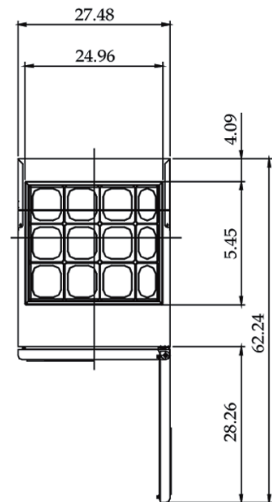
TST-28SD-12 PLAN VIEW
