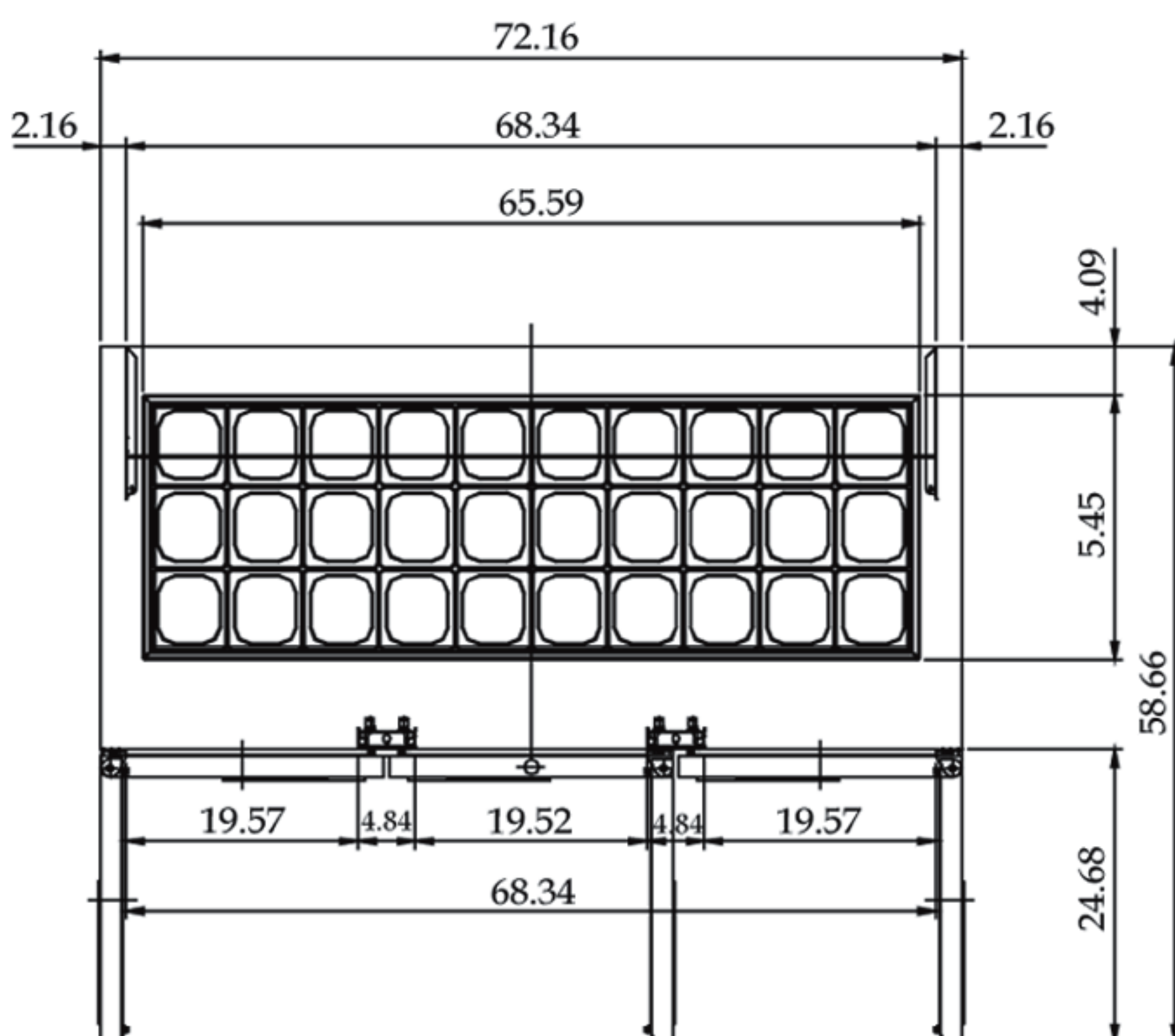
TST-72SD-30 PLAN VIEW
